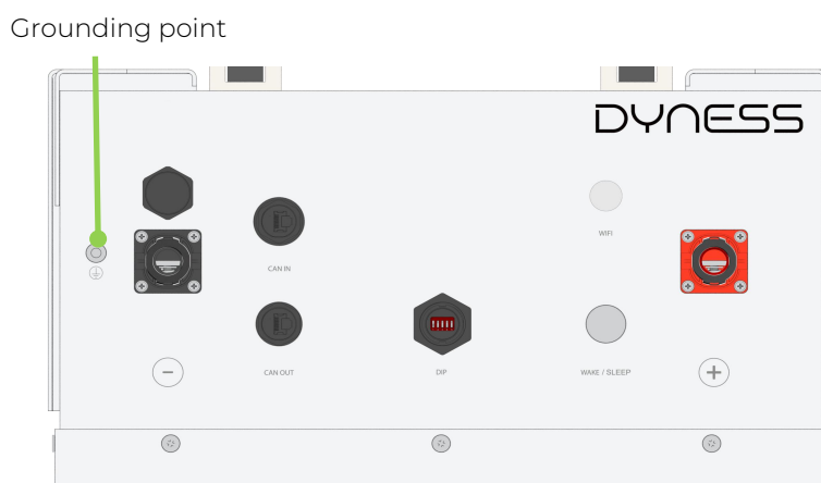
Figure 3-4 Location of grounding point
